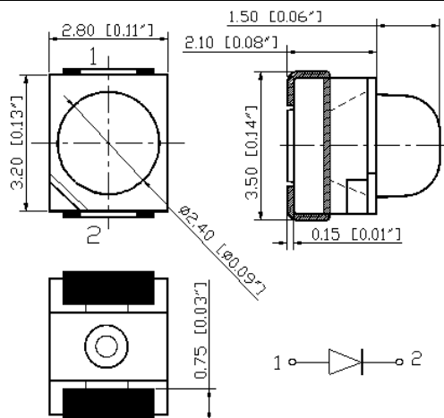
Package Dimensions (mm)
